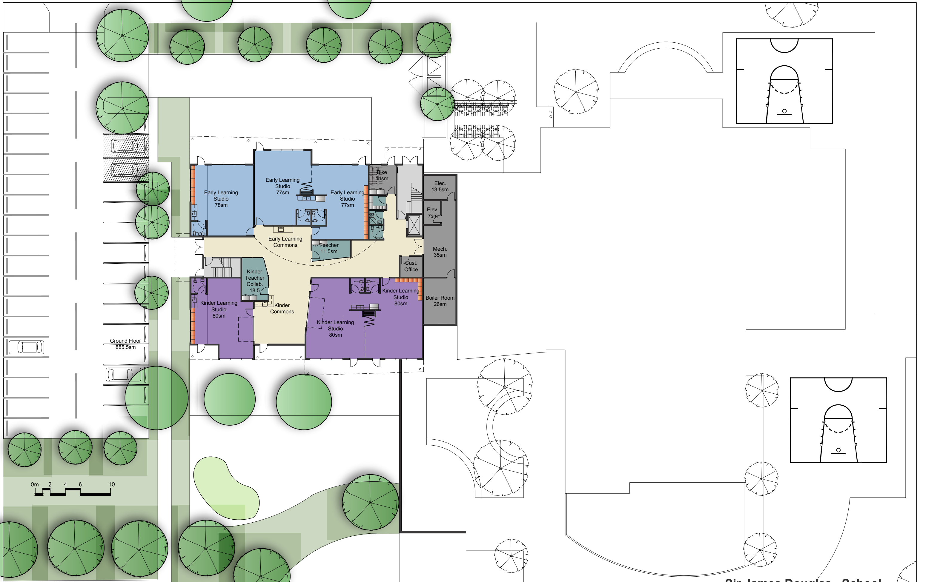
Sir James Douglas School Ground Floor Layout
